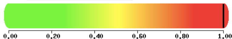
Figure V: Polyphen Analysis: Prediction of mutation specificity and sensitivity
