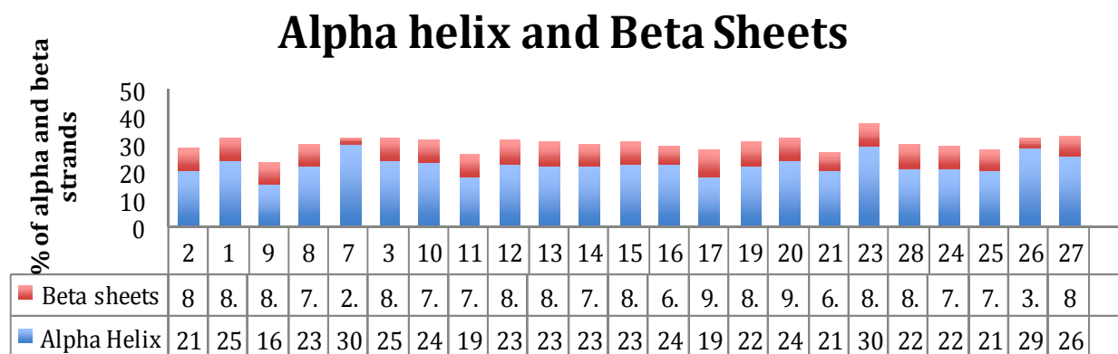
Figure III :Graphical representation of Alpha helix and beta sheets composition in MMPs
