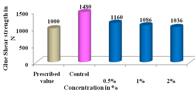
Fig II: Effect of Lufenron on Glue Shear strength of Wet Sample
