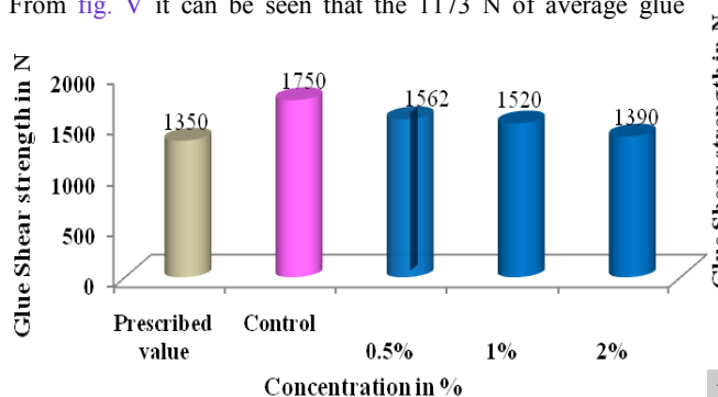
Fig I: Effect of Lufenron on Glue Shear strength of Dry Sample
