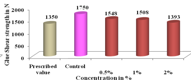
Fig VI: Effect of Diflubenzuron on Glue Shear strength of Dry Sample
