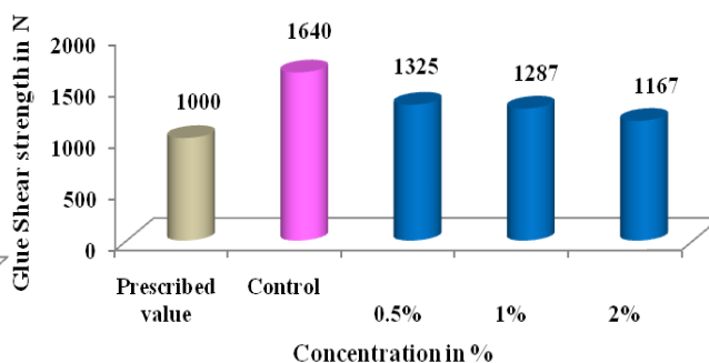
Fig III: Effect of Lufenron on Glue Shear strength of Mycological Sample
