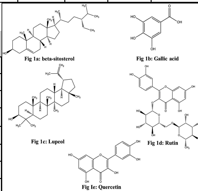
Fig I (a-e) : Compounds detected in methanolic flower extract characterized based on retention time (Fig. 2a and 2b). Our results are in agreement with the previous report of Bairagi et al. (2012) 29 . The comparative standard extract
